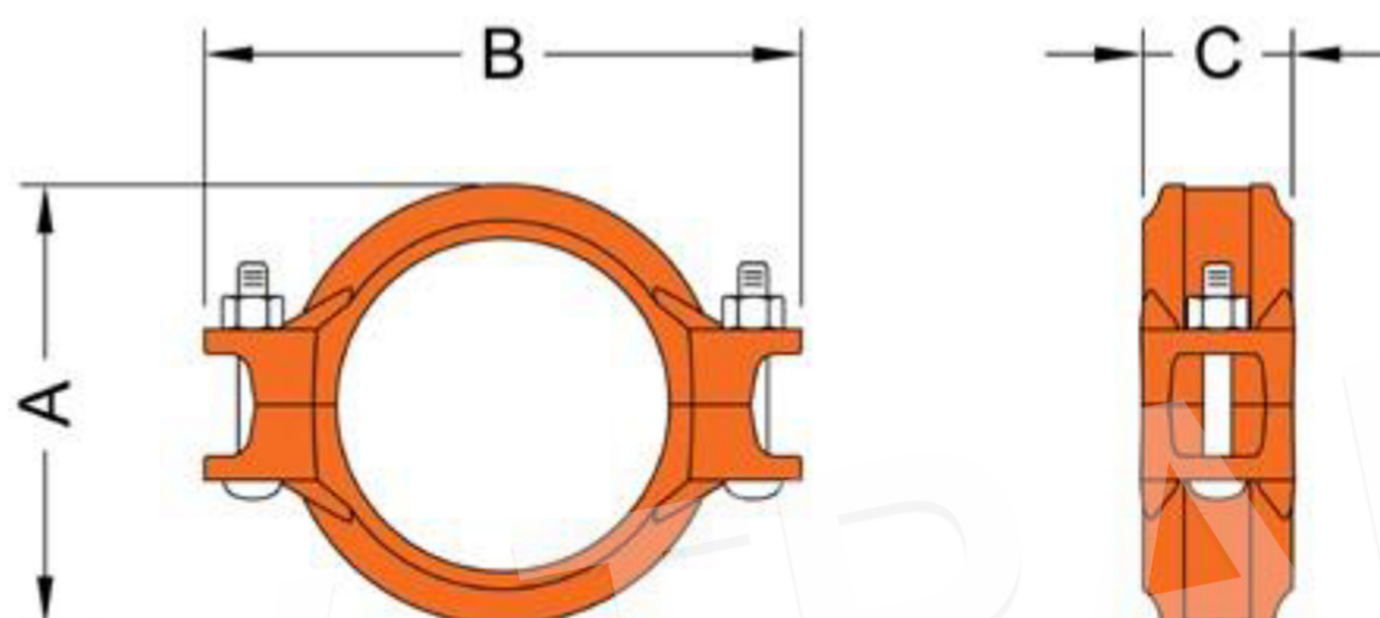
Model 7705 Standard Flexible Coupling
